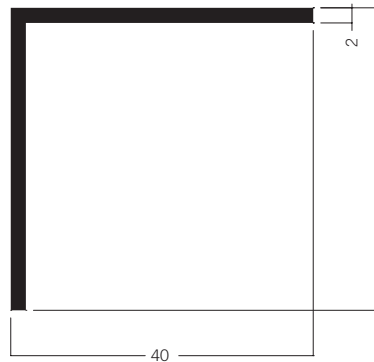
SO 400 Sockelwinkel OCTAeco floor 2.16 kg | 5000 mm
