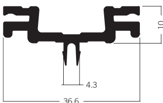
C 160 Adapterprofil 10 × 37 mm 1.61 kg | 6000 mm
