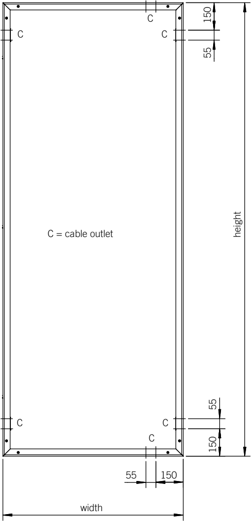
Positioning of cable outlets
