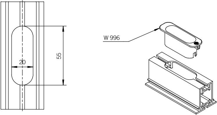
Cable outlet and cable protection
