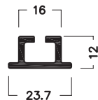
ADAPTOR EXTRUSION M 1311 (5000 mm)
