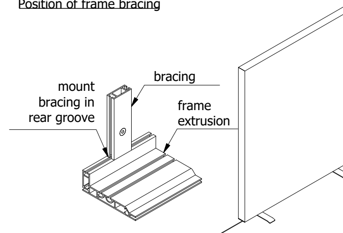
Position of frame bracing
