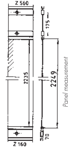
④ S_H-231 = Panel height
