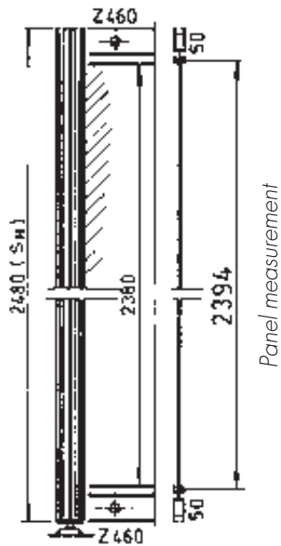
① S_H-86 = Panel height
