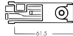
Tension lock Z 961/13 New: twin-grip lock
