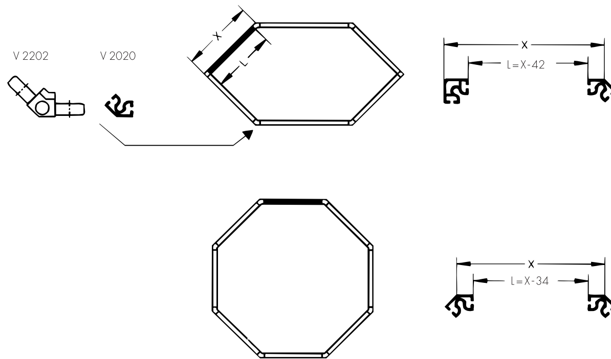
Cutting lengths for frame extrusions V 2100
