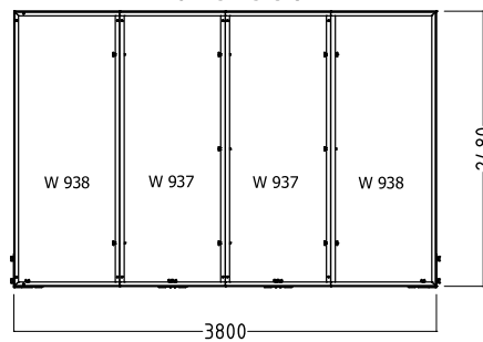
4 frame version
