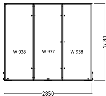
3 frame version
