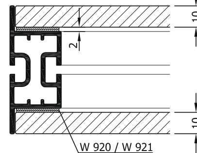
octawall 60 version 1 panel: 10mm hook-and-loop-tape: 2mm
